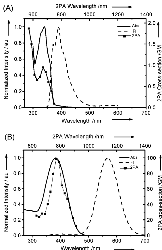
Figure 1. Absorption (solid line), emission (dashed line), and two-photon absorption (squares) spectra of (A) protonated form 1cH + (in pH 4 buffer) and (B) neutral form 1c (in pH 10 buffer). The absorption and fluorescence spectra are normalized.
