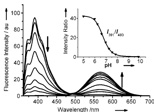
Figure 3. pH-dependence of the fluorescence intensity of 1c in buffer ( 10^{-5} \text{ M} ) excited at 355 nm (absorption isobestic point wavelength in Figure 2) with arrows indicating the change of the fluorescence intensities with pH increase. (Inset) Ratiometric calibration curve of I_{391}/I_{493} (intensity at 391 nm vs intensity at isoemissive point 493 nm).
